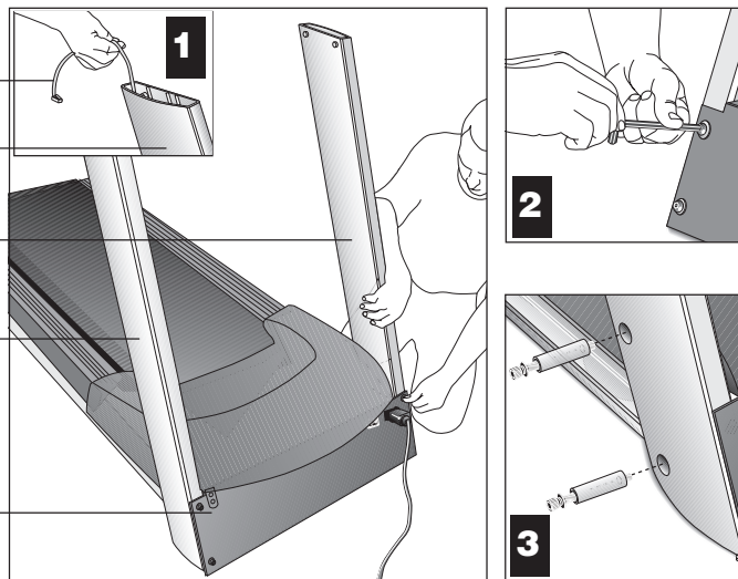
Diagram 6 Attach the upright supports.
