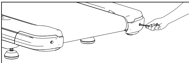
Figure 35: Location of the adjustment bolt
