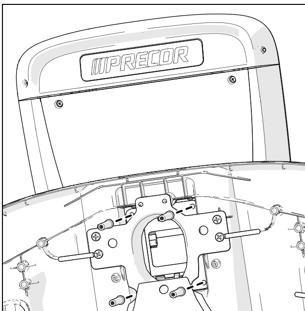
Figure 29: Securing the console
