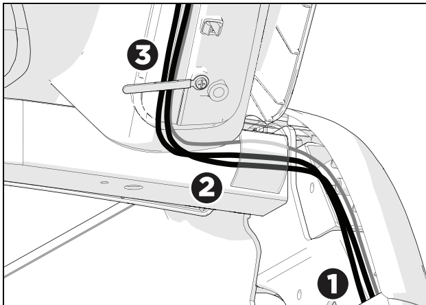
Figure 12: Console cable assembly positioning
