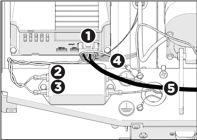
Figure 7: P80 power harness connection points
