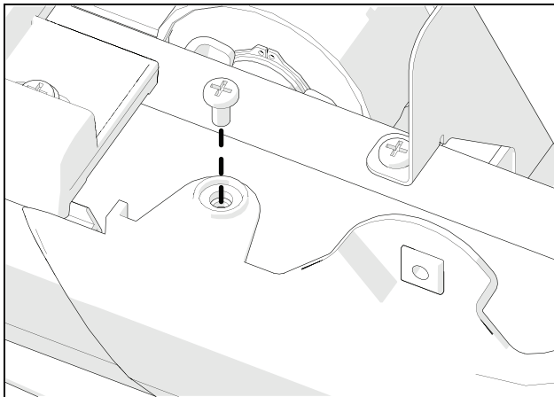
Figure 17: Corner cover attachment
