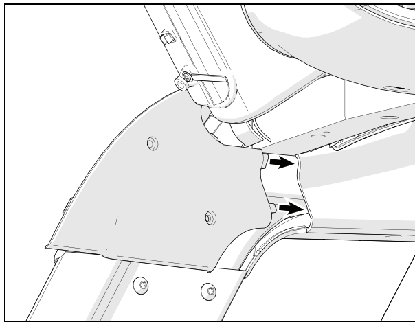
Figure 30: Access panel positioning
