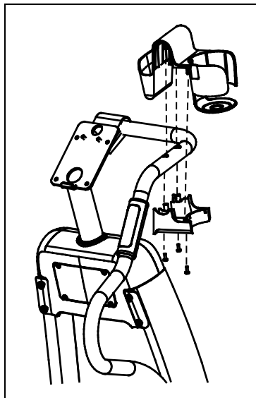
Figure 19: Water bottle attachment
