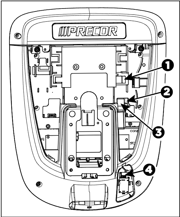
Figure 31: Cable connections, P30 console
