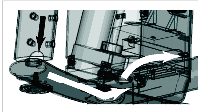
Figure 5: EFX cable path
