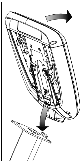
Figure 30: Console positioning on base unit
