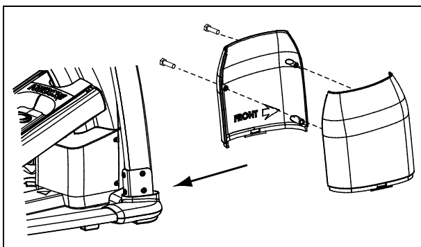
Figure 20: Upright support cover attachment (right-hand cover shown)
