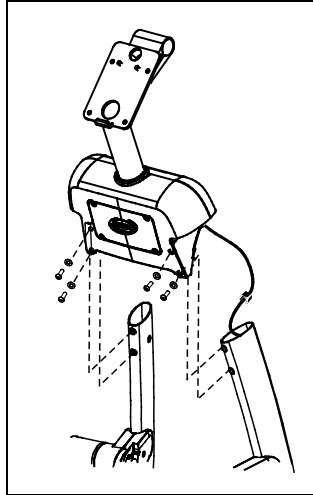
Figure 9: Attachment of center column support
