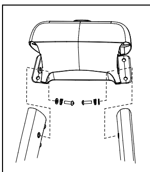
Figure 8: Rear view of console attachment
